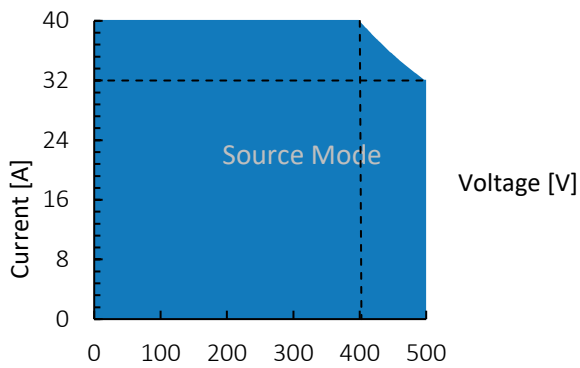
Figure 1: TC.P.16.500.400.S, voltage / current operating area.
