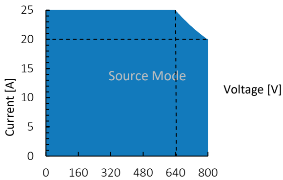
Figure 1: TC.P.16.800.400.S, voltage / current operating area.
