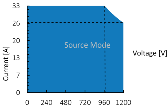
Figure 1: TC.P.32.1200.400.S, voltage / current operating area.
