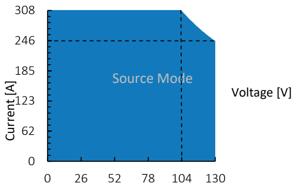
Figure 1: TC.P.32.130.400.S, voltage / current operating area.
