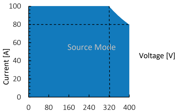
Figure 1: TC.P.32.400.400.S, voltage / current operating area.
