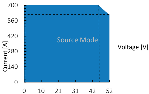
Figure 1: TC.P.32.52.400.S, voltage / current operating area.
