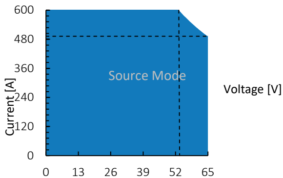
Figure 1: TC.P.32.65.400.S, voltage / current operating area.
