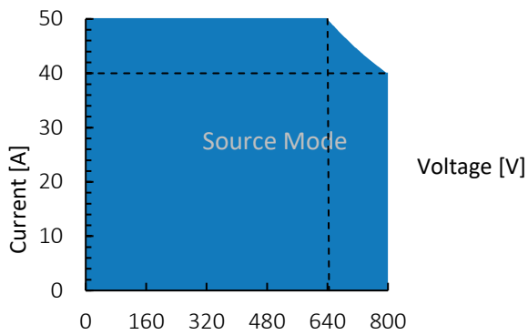
Figure 1: TC.P.32.800.400.S, voltage / current operating area.
