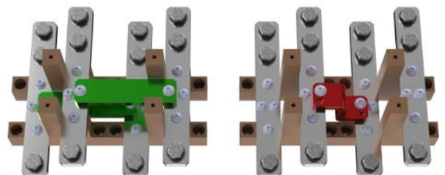
Figure 5: The DC switch panel offers high-quality jumper bars for parallel and series/matrix connection. Together with the comfortable reconfiguration tab in the G5.Control operating and service software, the current or voltage range of the G5 power system can be doubled or tripled within a very short time.
