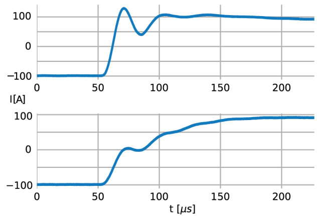
Figure 2: Parameterization example: of a 36 kW, 1000 V, 108 A device: Set-value step current -97...97 A@333VDC in <50 \mu\text{s}</math> with overshoot (top), in <200 \mu\text{s}</math> w/o overshoot (bottom). The dynamic behavior is comparable across the series of G5 devices from low voltage to high voltage
